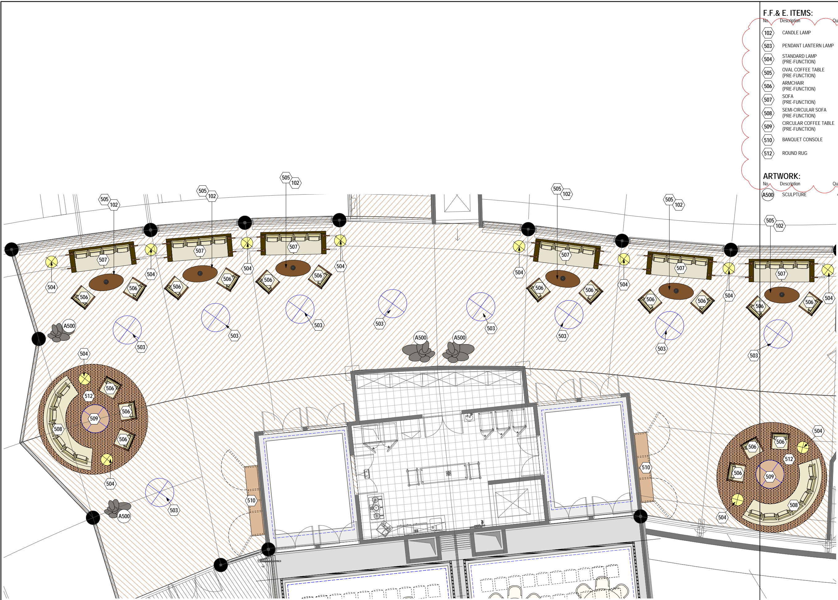
1 PRE FUNCTION FFE PLAN Scale 1:100 @ A3
